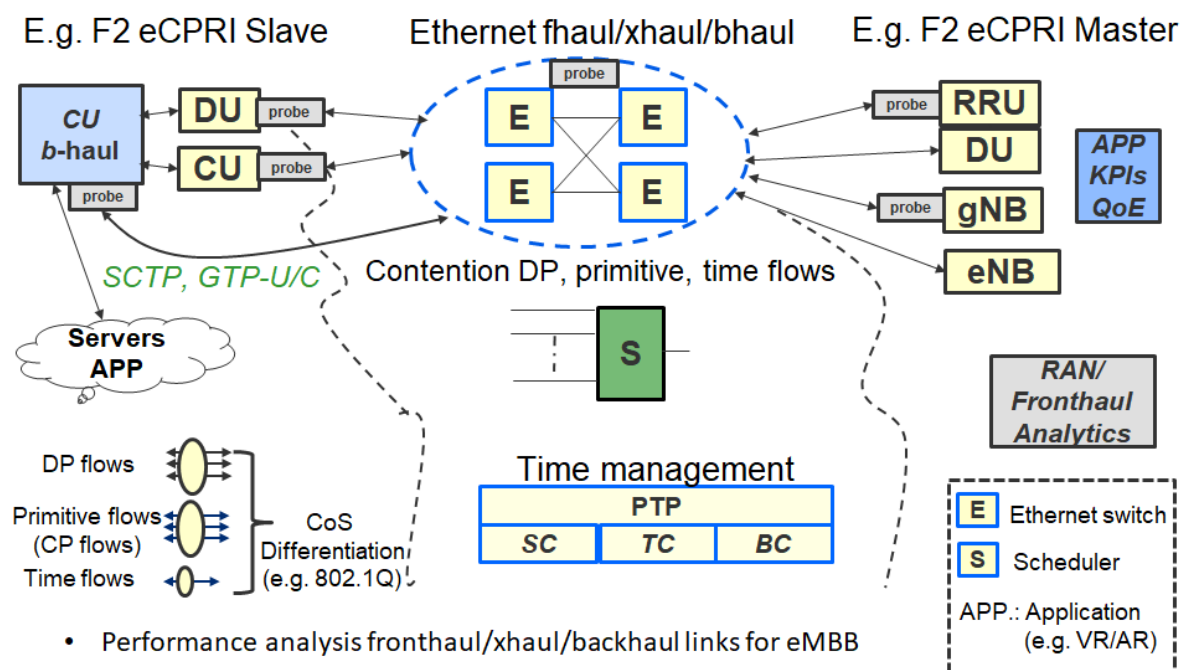
Figure 19: Overview of test domains within the fronthaul, x-haul and/or backhaul links. PTP, Precision Time Protocol; SC, Slave Clock; TC, Transport Clock; BC, Boundary Clock; APP, Application; DP, Data Plane. DU, Distributed Unit; CU, Central Unit; RRU, Remote Radio Unit.
